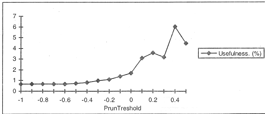
FIGURE 3 - PrunThreshold X Usefulness ratio (Motivo de cobrança)
