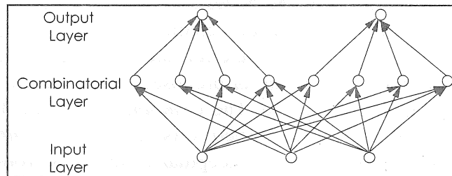
FIGURE 1 - CNM neural network
